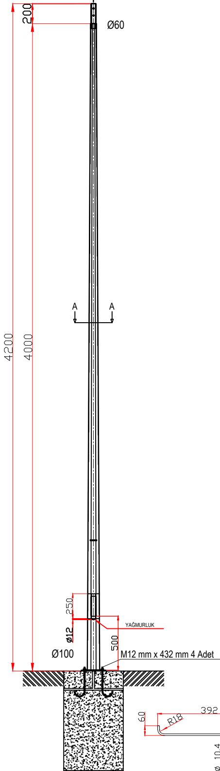
ANCHOR BOLTS M12*432
