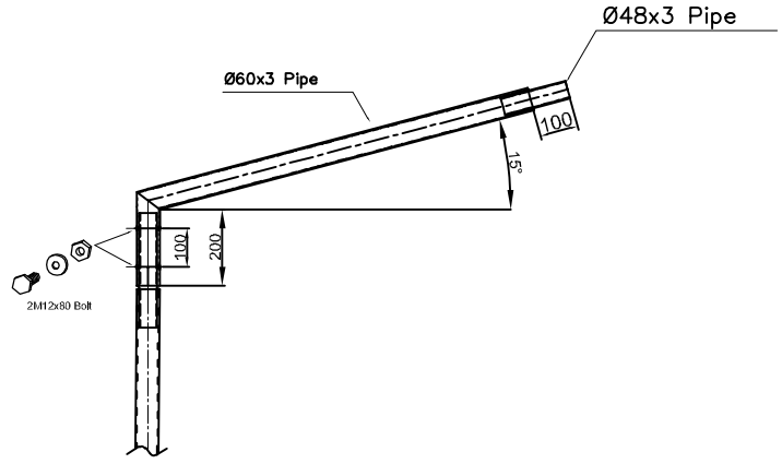
FRONT VIEW OF SINGLE ARM
