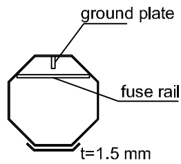
B-B SECTION
