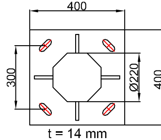
BASE PLATE C-C SECTION
